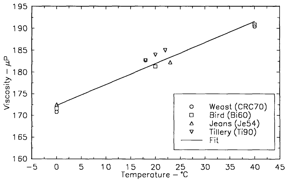
Figure III-33. A plot of air viscosity measurements in the temperature range from 0° C to 40° C and a linear fit of these data.
