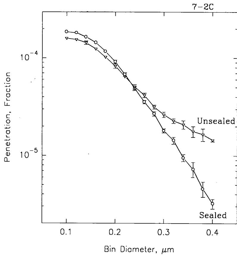
Figure V-1. Penetration data showing a reduction in penetration at bin diameters greater than \approx 0.3 \mu\text{m} when the filter unit frame is sealed. Filter unit operating at Q_{de} .
