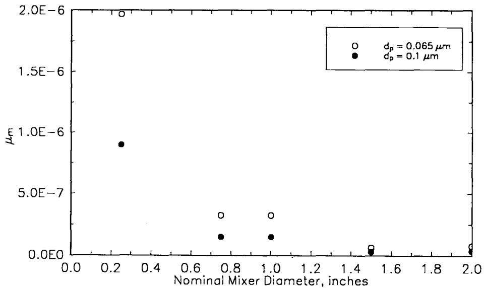
Figure III-24. Results of diffusion loss analysis showing values of \mu_m for d_p = 0.065 \mu\text{m} and 0.1 \mu\text{m} .
